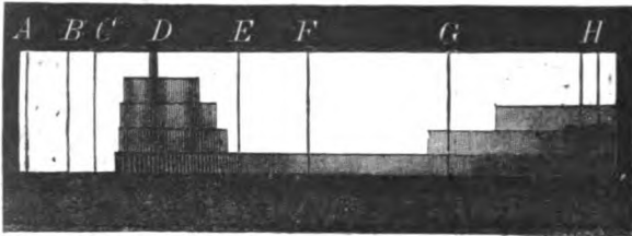
FIG. 4.—Absorption of colouring matter of litmus.
